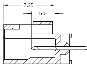
SECTION Z-Z
