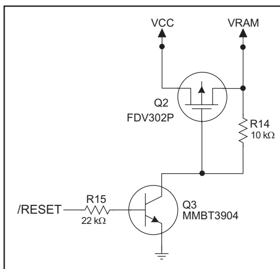
Figure C-3. VRAM Switch
