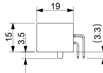
SECTION Z-Z
