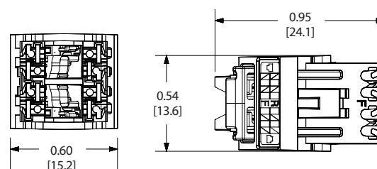
45° Angled Up/Down Wire Cap Assembly
