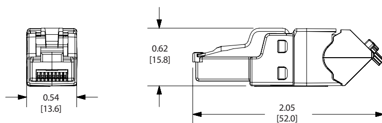
45° up/down Angled Field Term Plug w/out protective cover
