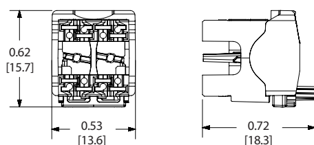
Straight Wire Cap Assembly
