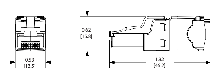
Straight Field Term Plug w/out protective cover
