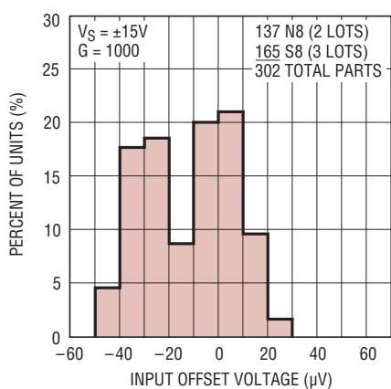
Distribution of Input Offset Voltage, T_A = 25^\circ\text{C}
