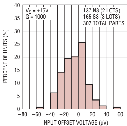
Distribution of Input Offset Voltage, T_A = -40^\circ\text{C}
