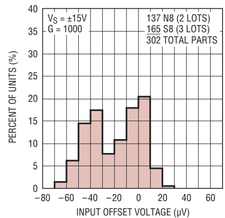
Distribution of Input Offset Voltage, T_A = 85^\circ\text{C}
