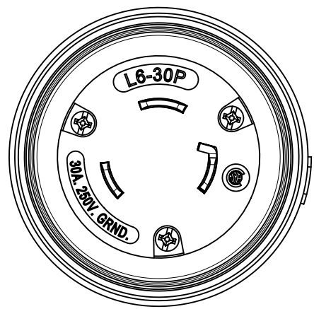
NEMA L6-30 PRIMARY WOODHEAD #28W48 PLUG COLOR-YELLOW
