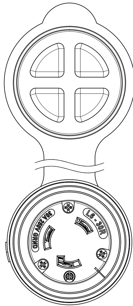
NEMA L6-30 SECONDARY WOODHEAD #29W48 CONNECTOR COLOR-YELLOW
