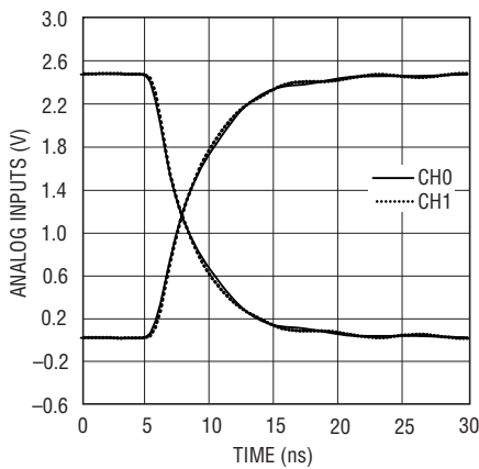
Simultaneous Input Steps at CH0 and CH1 from 25Ω
