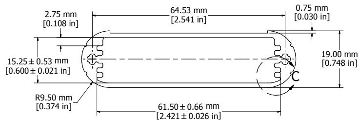
EXTRUSION
