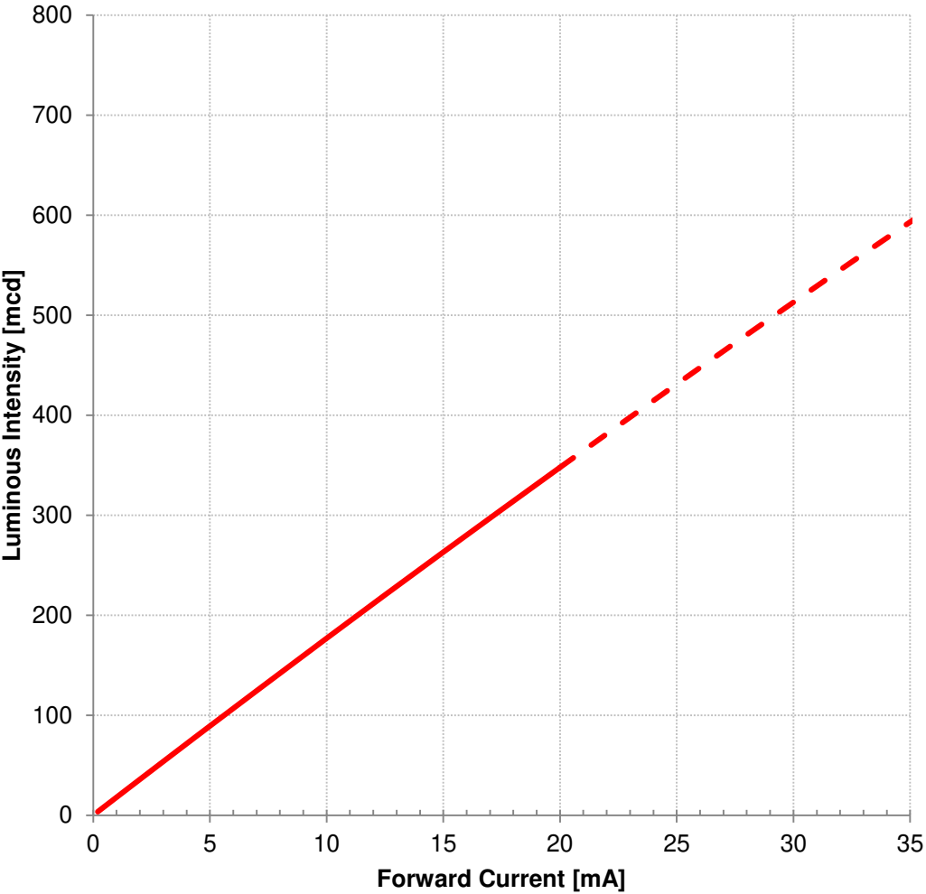
Luminous Intensity vs. Forward Current:
