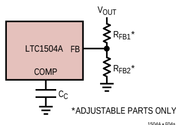
Figure 4a. Minimum Compensation Network
