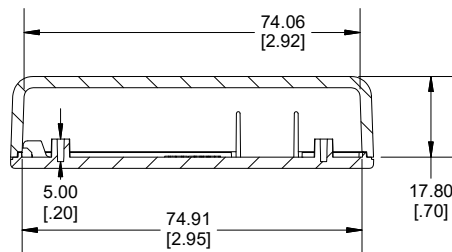
SECTION B-B END VIEW
