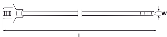
T50SOS2DOP
