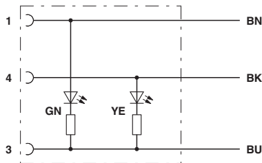
Contact assignment of M8 socket with 2 LEDs
