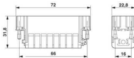
Male insert
