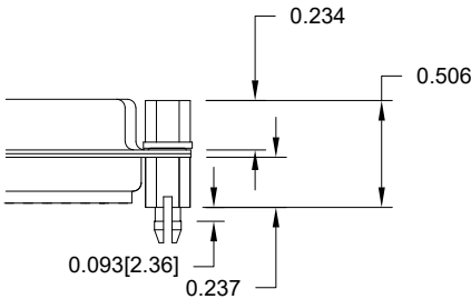
92X ..... 0.237" (BOARD SIDE)
