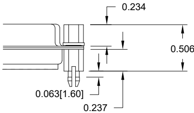
91X ..... 0.237" (BOARD SIDE)
