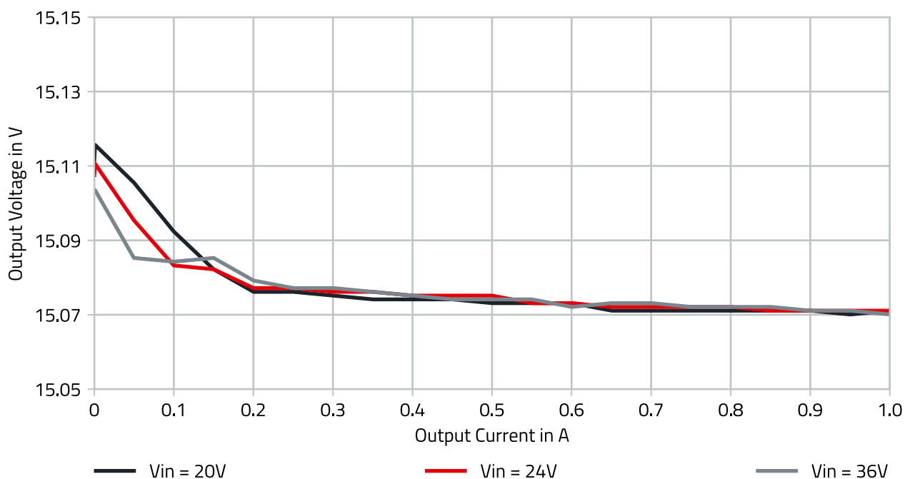
Figure 6: Load regulation.
