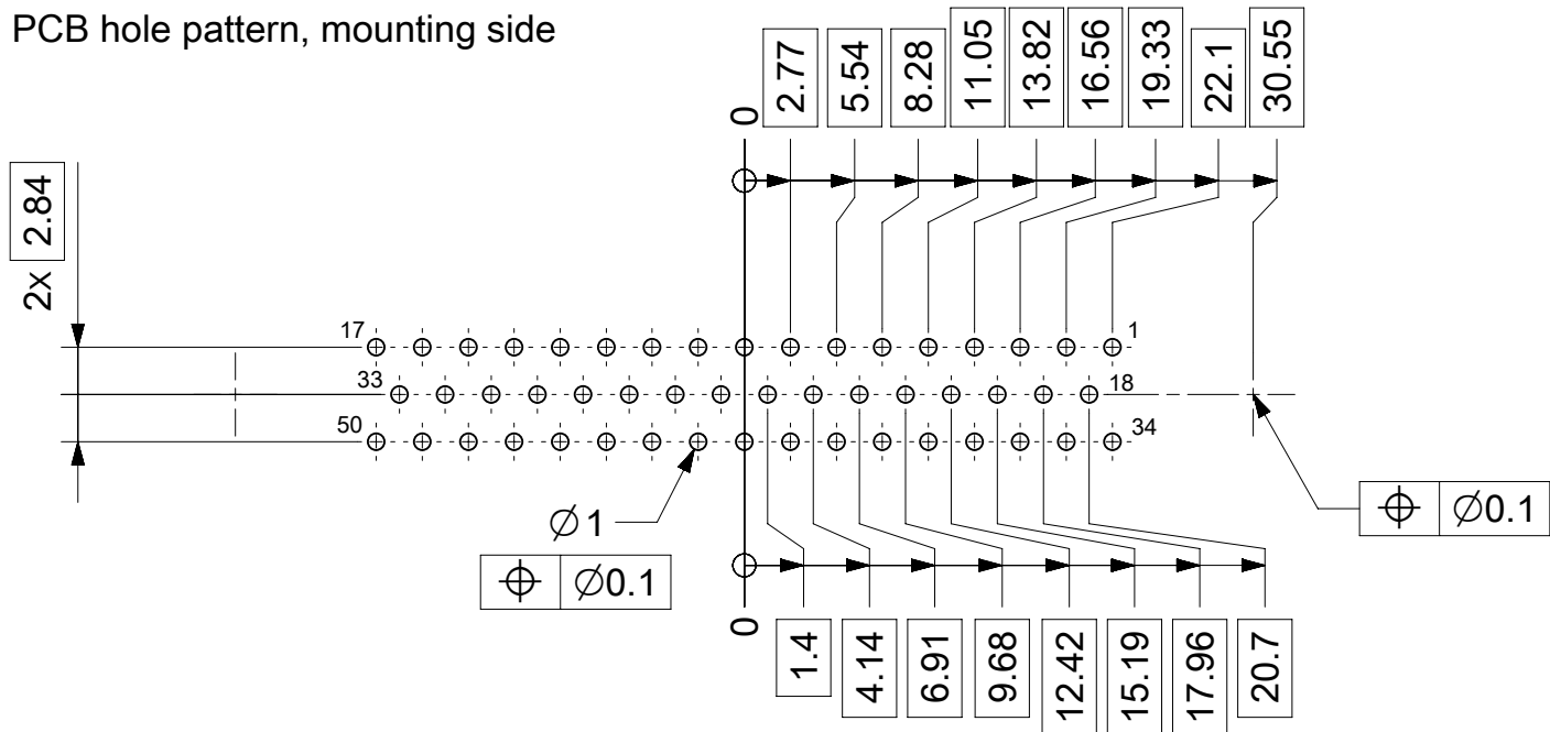
PCB hole pattern, mounting side
