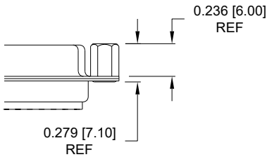
03 ..... 0.236" MATING SIDE
