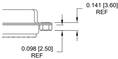
S5 ..... 0.237" BOARD SIDE
