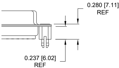
S5 ..... 0.237" BOARD SIDE
