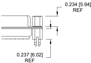
95 ..... 0.237" BOARD SIDE 0.234" MATING SIDE
