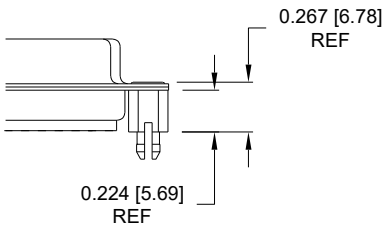
05 ..... 0.224" BOARD SIDE
