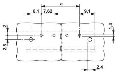
Drilling diagram
