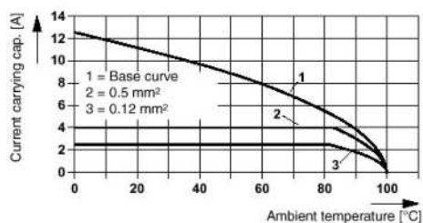
FK-MPT 0,5-ST-3,5 with PST 1,0
