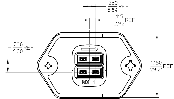
RECOMMENDED PCB LAYOUT COMPONENT SIDE
