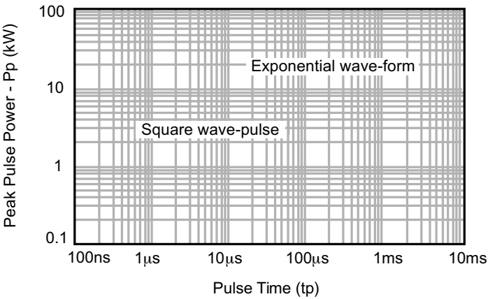
Figure 3 - Peak Pulse Power vs. Pulse Time
