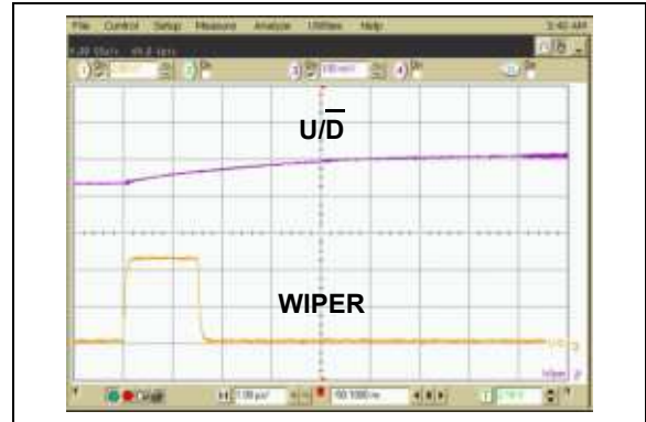
FIGURE 2-47: 50 k \Omega – Low-Voltage Increment Wiper Settling Time ( V_{DD} = 5.5\text{V} ).
