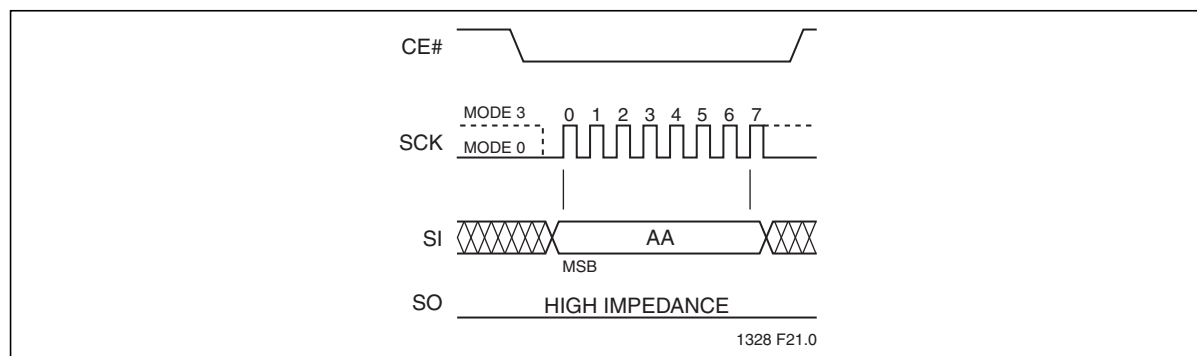
Figure 21: Enable-Hold Sequence
