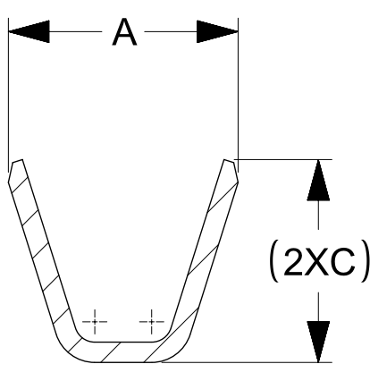
SECTION Y-Y
