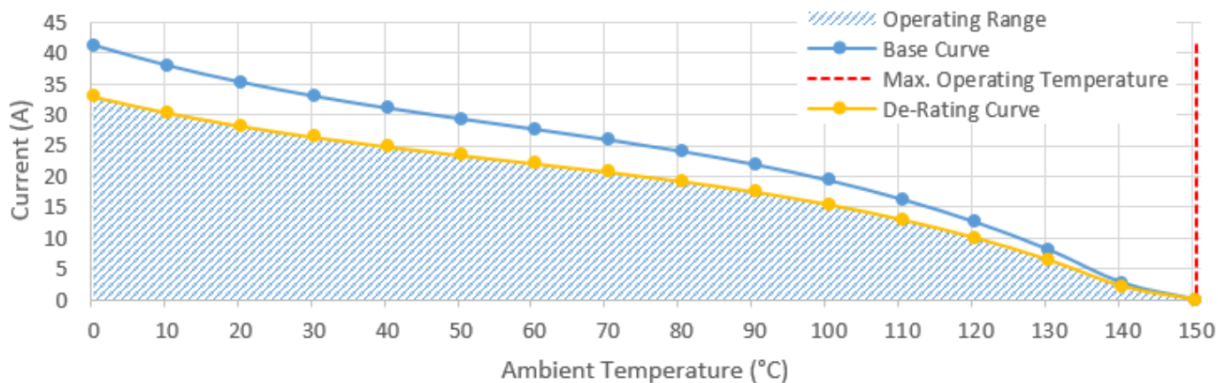
CURRENT CARRYING CAPACITY: 16 AWG
