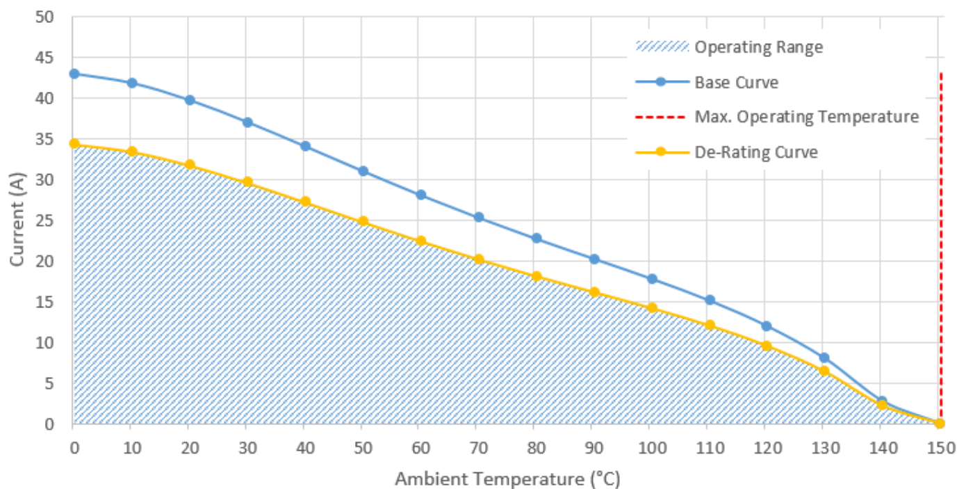
CURRENT CARRYING CAPACITY: 18 AWG
