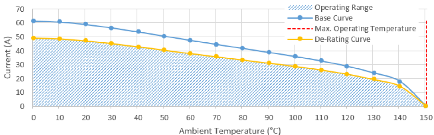
CURRENT CARRYING CAPACITY: 12 AWG
