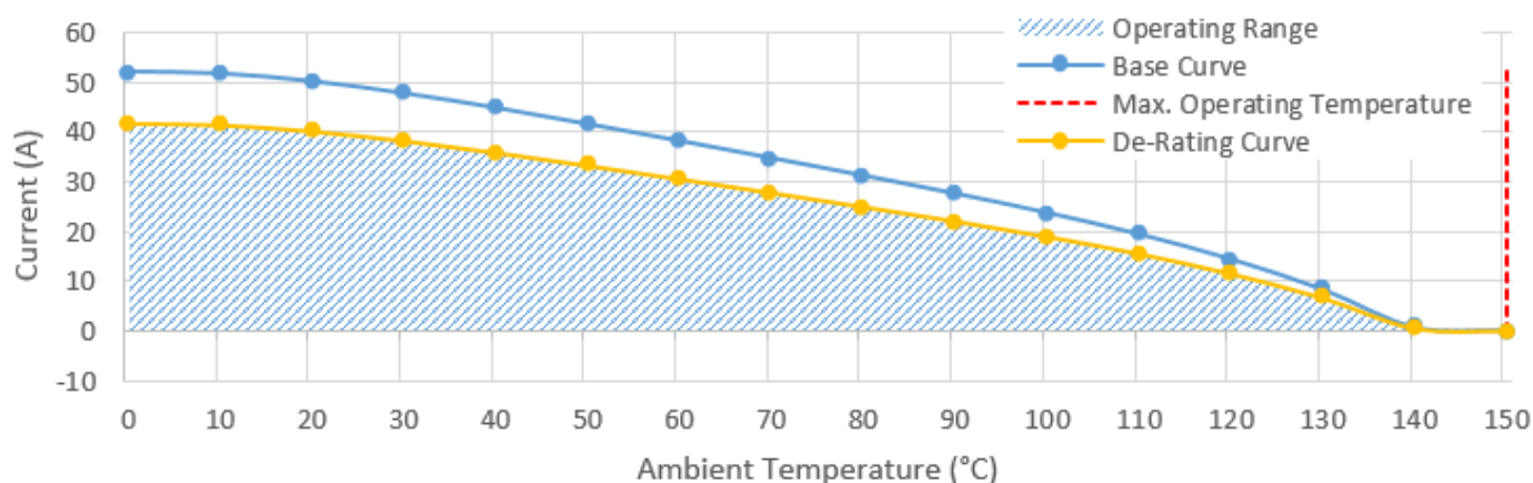
CURRENT CARRYING CAPACITY: 14 AWG
