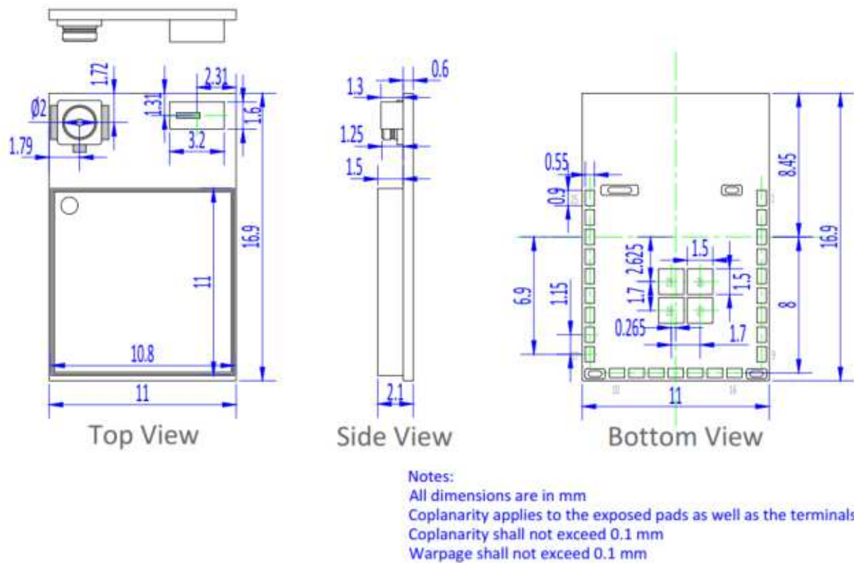
Figure 6-1. Mechanical Drawing
