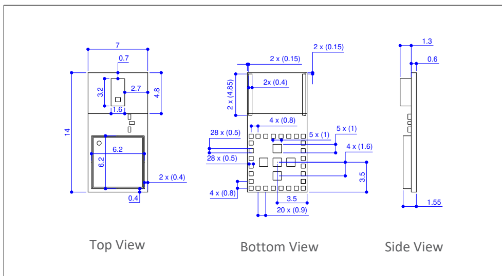
Figure 4-1. Mechanical Drawing
