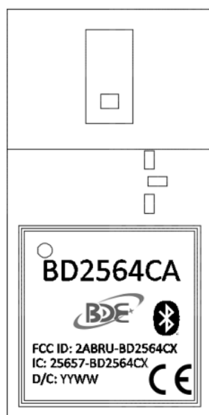
Figure 5-1. Module Marking
