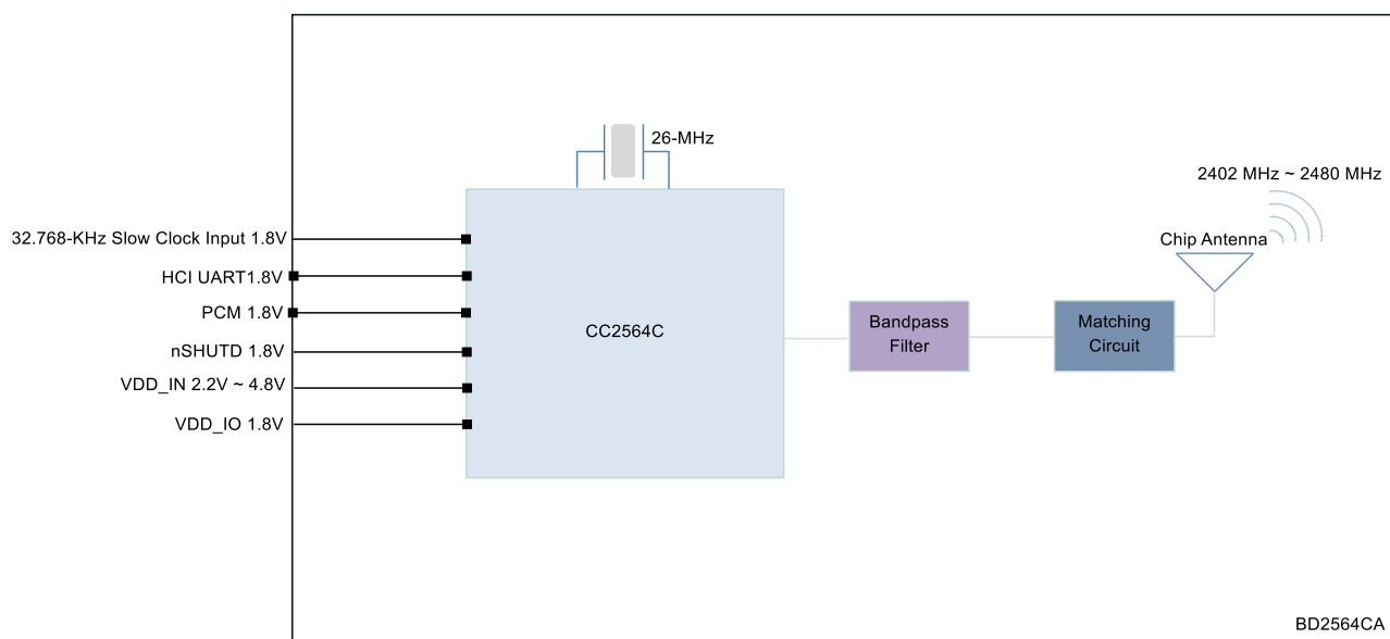
Figure 1-1. The block diagram of BDE-BD2564CA
