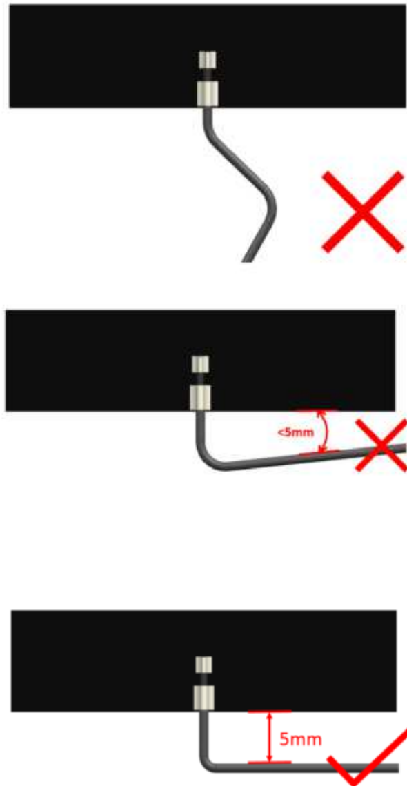
FIGURE 5.2.1 CABLE BENDING
