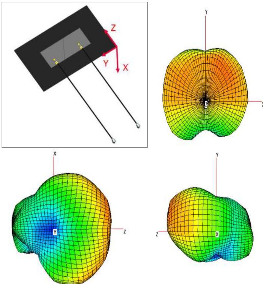
FIGURE 4.6.2 3D RADIATION PATTERN OF ANTENNA AT 5500MHZ BAND OF PORT 1 IN FREE SPACE
