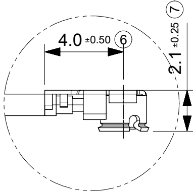
DETAIL A SCALE 5:1 CONNECTOR
