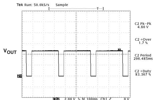
Thermal Shutdown Response of 5.0V LDO
