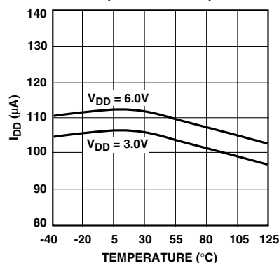
I DD vs. Temperature (SELECT = NC)
