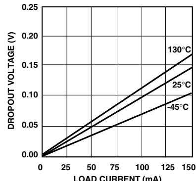
Dropout Voltage2 vs. Load Current (SELECT = V DD )
