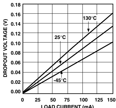
Dropout Voltage1 vs. Load Current (SELECT = V DD )
