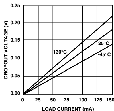
Dropout Voltage2 vs. Load Current (SELECT = V DD )
