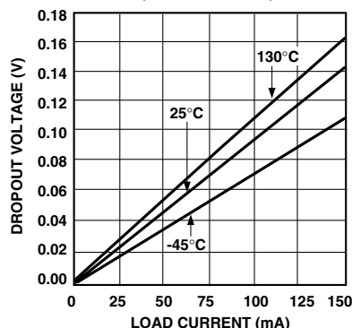
Dropout Voltage1 vs. Load Current (SELECT = NC)
