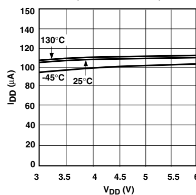
I DD vs. V DD (SELECT = GND)
