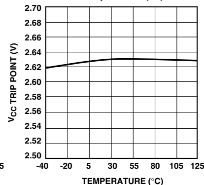
V CC Trip Point vs. Temperature (°C)
