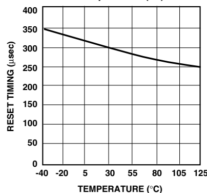
Reset Active Time vs. Temperature (°C)
