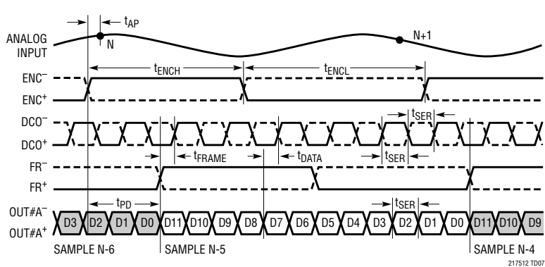
One-Lane Output Mode, 12-Bit Serialization
