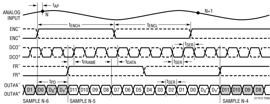
One-Lane Output Mode, 14-Bit Serialization
