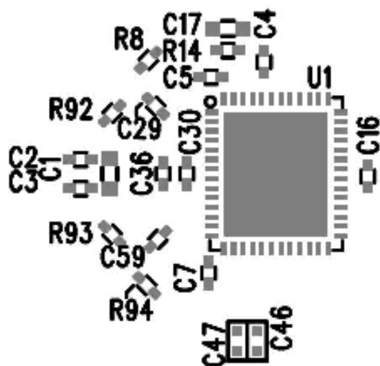
Silkscreen Top
