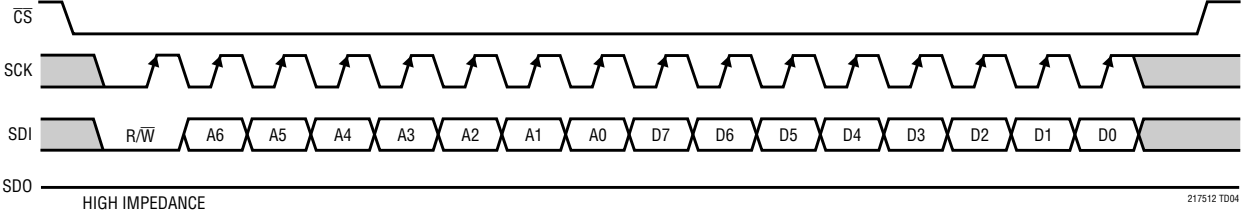
SPI Port Timing (Write Mode)
