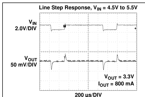
FIGURE 2-12: Line Transient Response.
