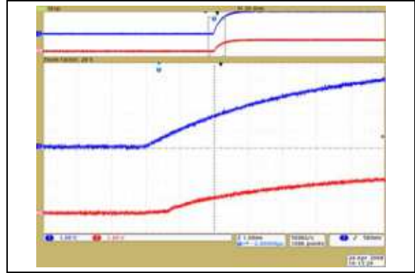
FIGURE 2-50: 50\text{ k}\Omega – Low-Voltage Increment Wiper Settling Time ( V_{DD} = 2.7\text{V} ) ( 1\text{ }\mu\text{s/Div} ).
