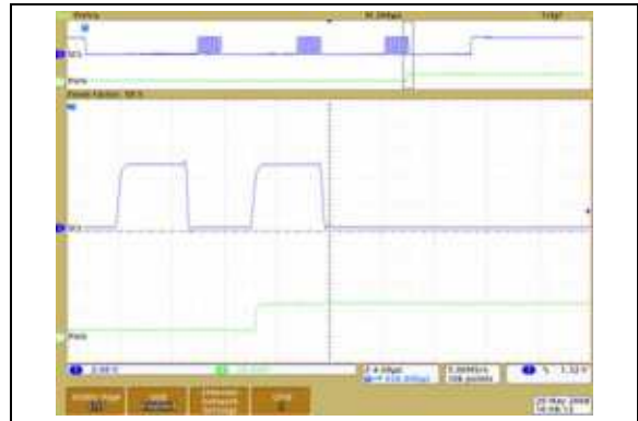
FIGURE 2-51: 50\text{ k}\Omega – Low-Voltage Increment Wiper Settling Time ( V_{DD} = 5.5\text{V} ) ( 1\text{ }\mu\text{s/Div} ).
