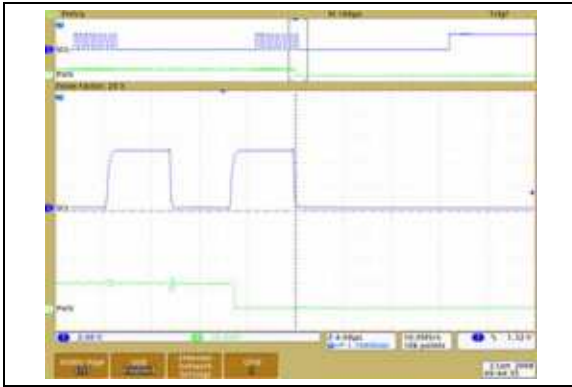
FIGURE 2-63: 100\text{ k}\Omega – Low-Voltage Decrement Wiper Settling Time ( V_{DD} = 2.7\text{V} ) ( 1\text{ }\mu\text{s/Div} ).
