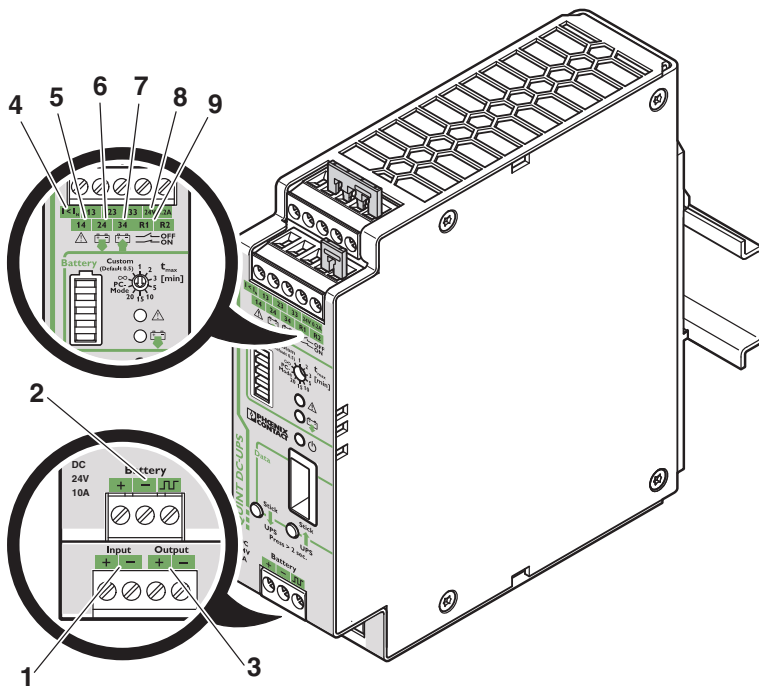
Figure 1 Connection terminal blocks
