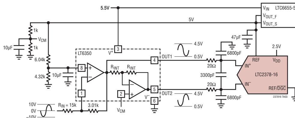
LT6350 Configured to Accept a \pm 10V Input Signal While Running Off of a Single 5.5V Supply When Digital Gain Compression Is Enabled in the LTC2378-16
