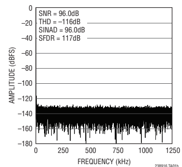
32k Point FFT f_{\text{SMPL}} = 2.5\text{Msps} , f_{\text{IN}} = 2\text{kHz}
