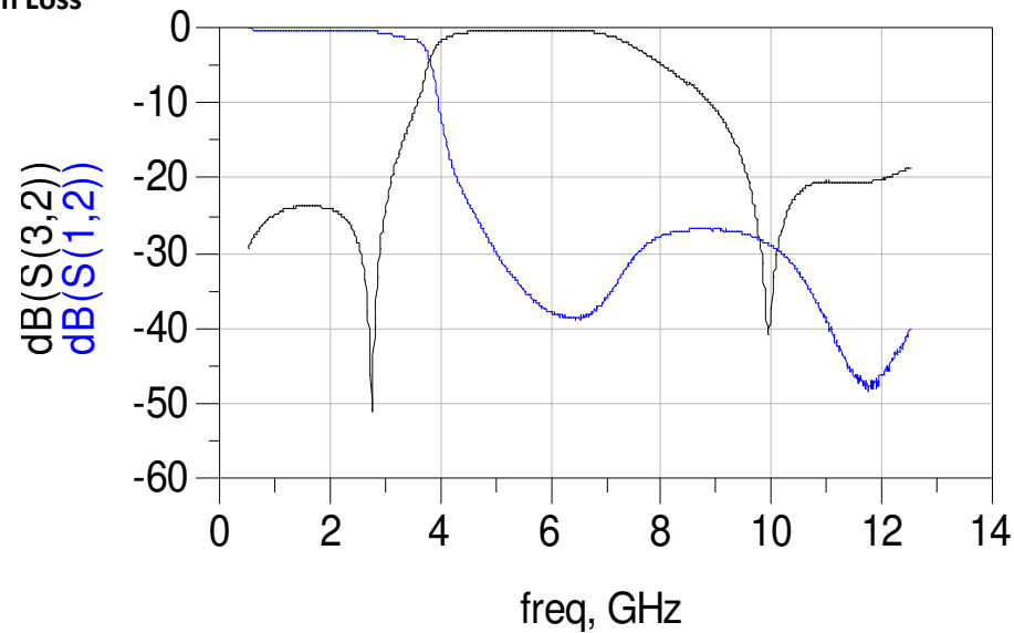
Insertion Loss
