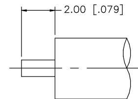
RECOMMENDED CABLE STRIPPING DIMENSIONS
