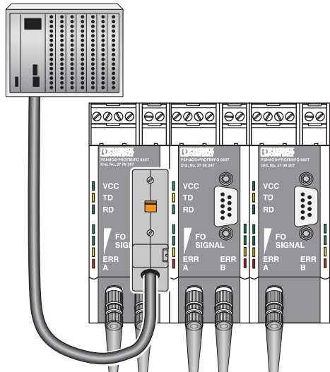
Figure 11 PROFIBUS interface
