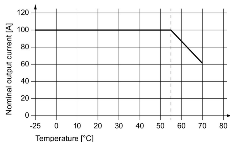
Temperature Derating
