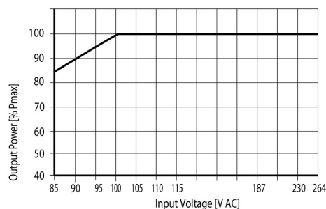
AC-Input Derating
