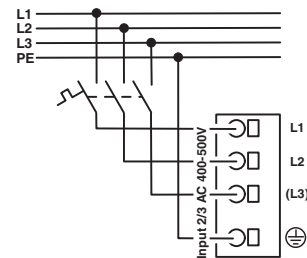
Figure 12 Schematic diagram, switching the input terminals
