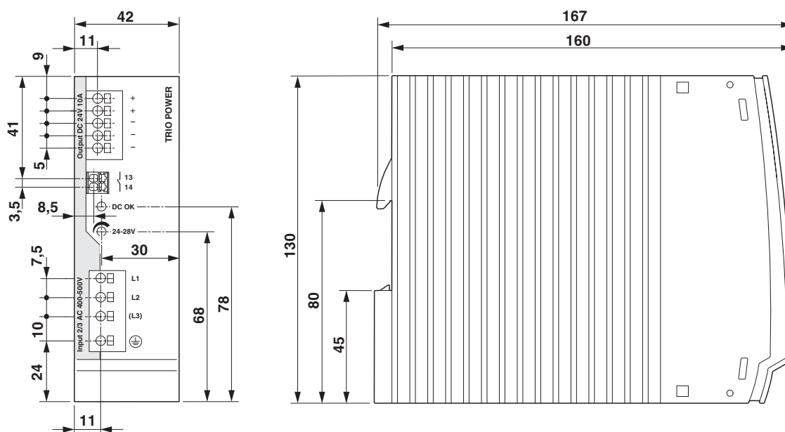
Figure 5 Device dimensions
