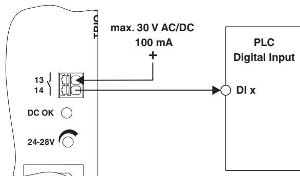
Figure 18 Wiring principle
