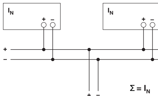
Figure 26 Schematic diagram in parallel operation
