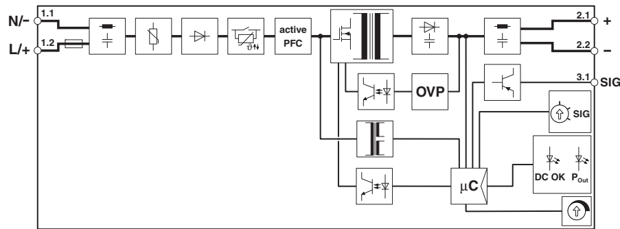
Figure 6 Block diagram
