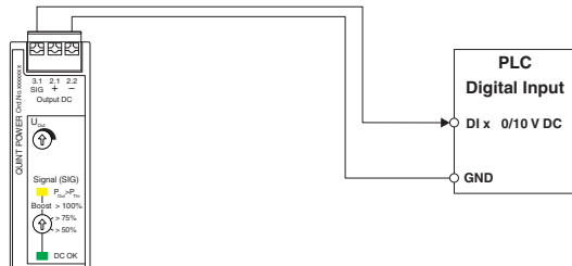
Figure 23 Signaling
