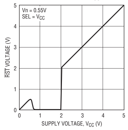
\overline{RST} Output Voltage vs V_{CC}
