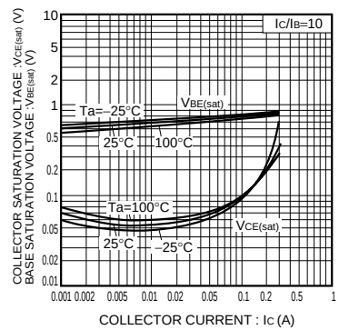
Fig.6 Collector-emitter saturation voltage vs. collector current Collector-base saturation voltage
