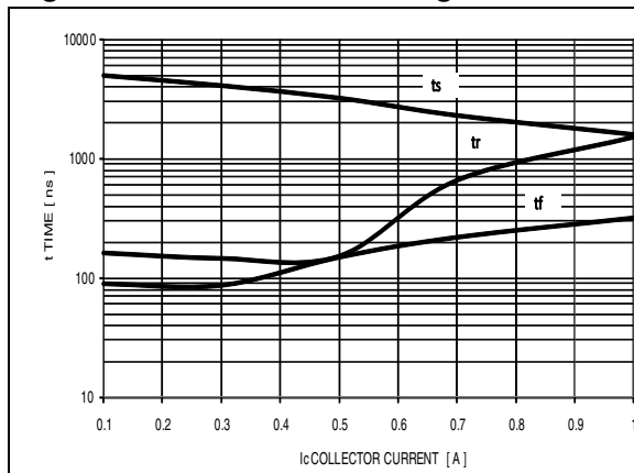
Figure 12. Resistive switching time
