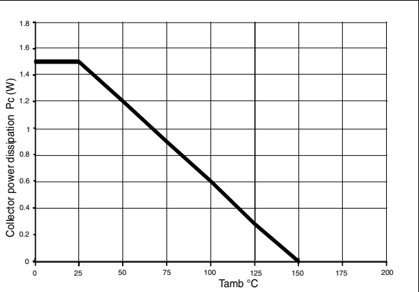
Figure 3. Derating curve
