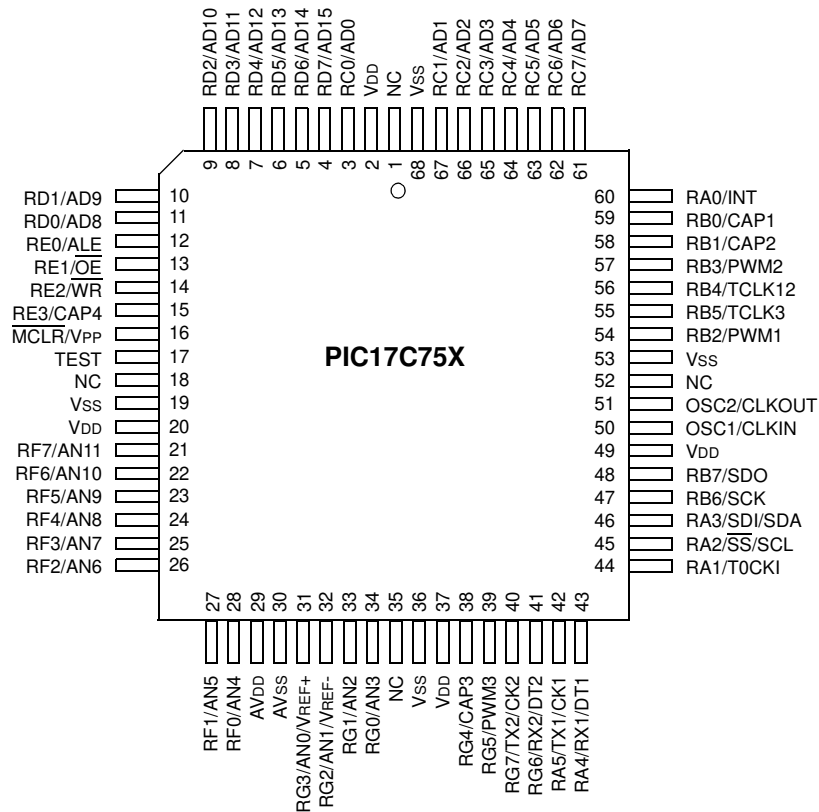
68-Pin PLCC
