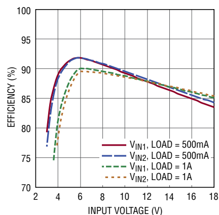
3.3\text{V}_{OUT} Efficiency vs V_{IN1} or V_{IN2} Voltage with 500mA and 1A Load Current
