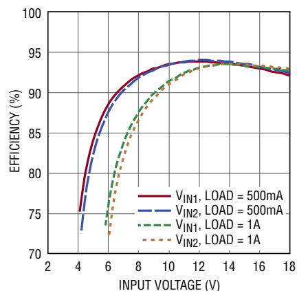
5\text{V}_{OUT} Efficiency vs V_{IN1} or V_{IN2} Voltage with 500mA and 1A Load Current
