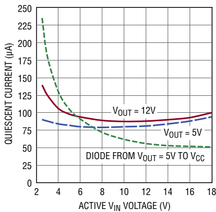
No-Load Active V_{IN} Current in Burst Mode
