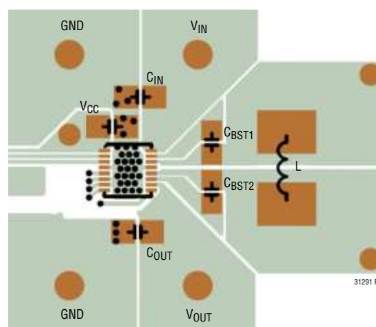
Figure 4. Typical 2-Layer PC Board Layout (MSE Package)
