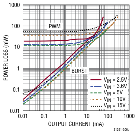
Power Loss, V_{OUT} = 6.9\text{V}
